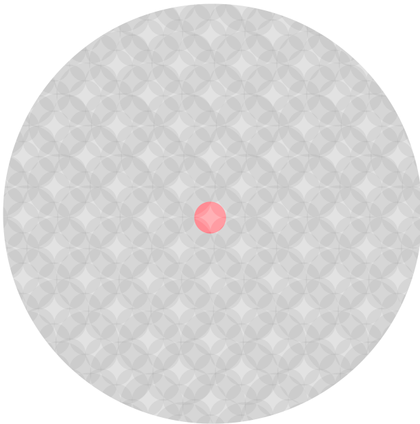
FIGURE 4.1. In G = \mathbb{R}^2 : Illustration of pattern formed by overlapping balls 2B_R with R \in \text{Near}(Q) inside of the window 40B_Q . The central region 2B_Q is highlighted.
